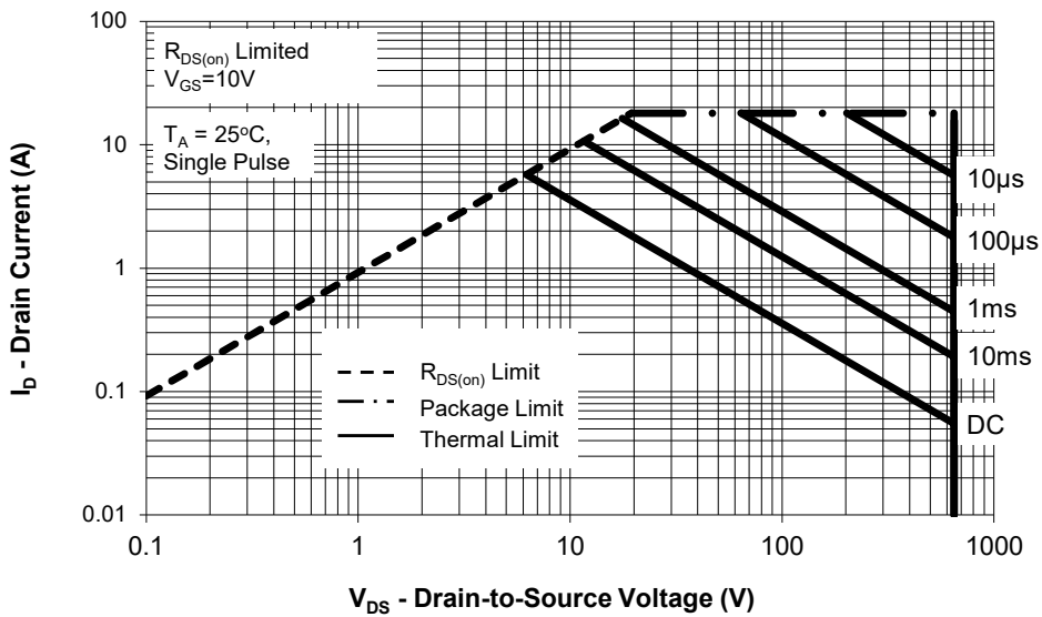
Full Pak TO-220 Package Maximum Rated Forward Biased SOA
