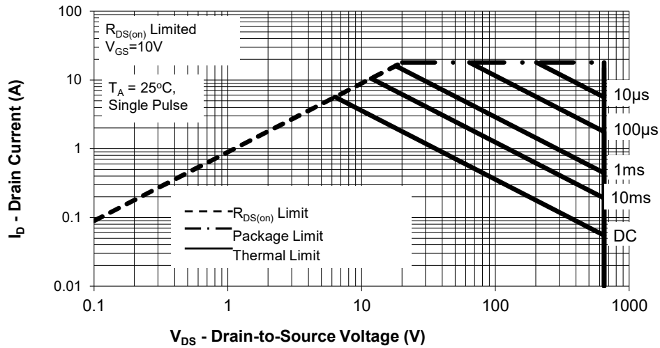
Full Pak TO-220 Package Maximum Rated Forward Biased SOA
