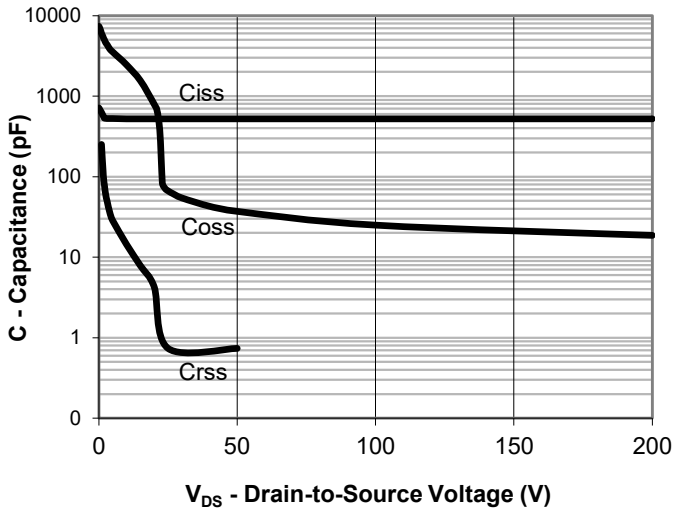
Capacitance
