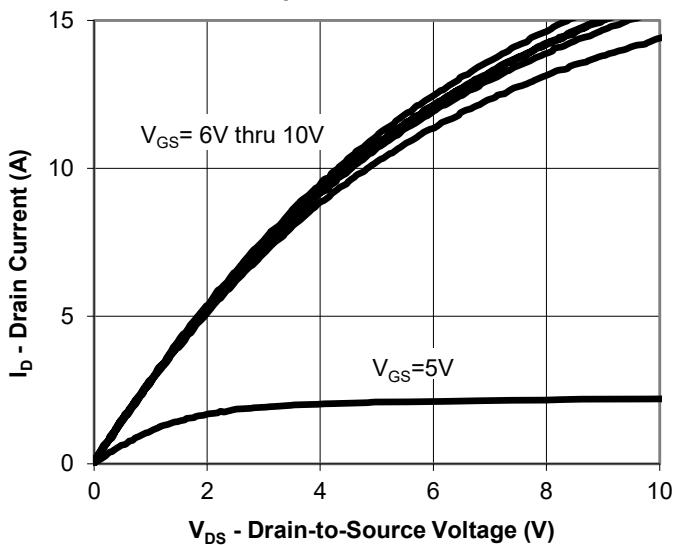
Output Characteristics
