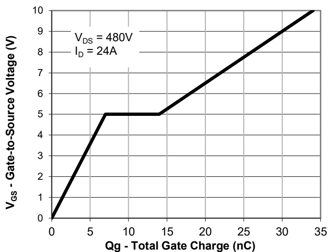
Gate Charge
