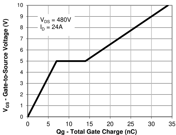
Gate Charge
