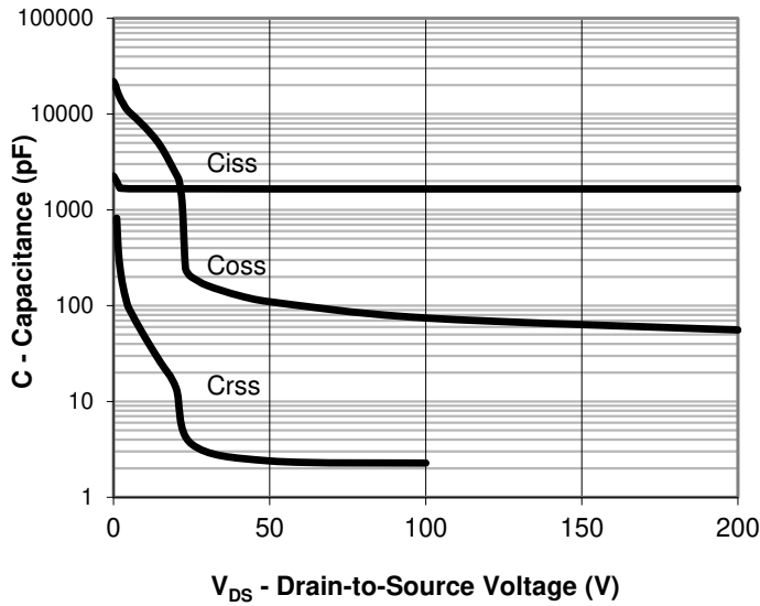
Capacitance
