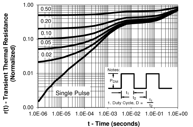
Full Pak TO-220 Transient Thermal Response, Junction-to-Ambient
