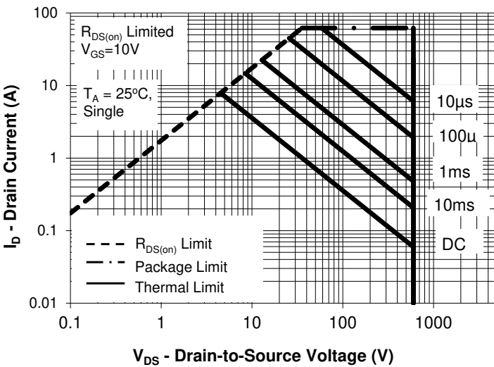
Maximum Rated Forward Biased SOA
