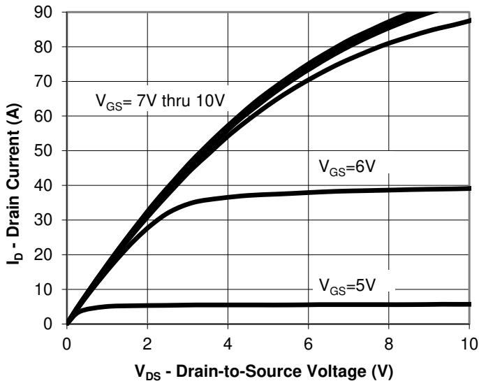
Output Characteristics
