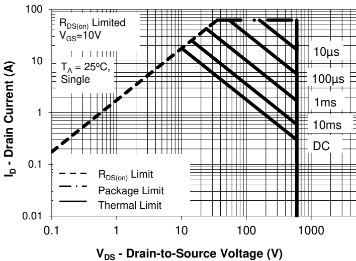
TO-247 Package Maximum Rated Forward Biased SOA
