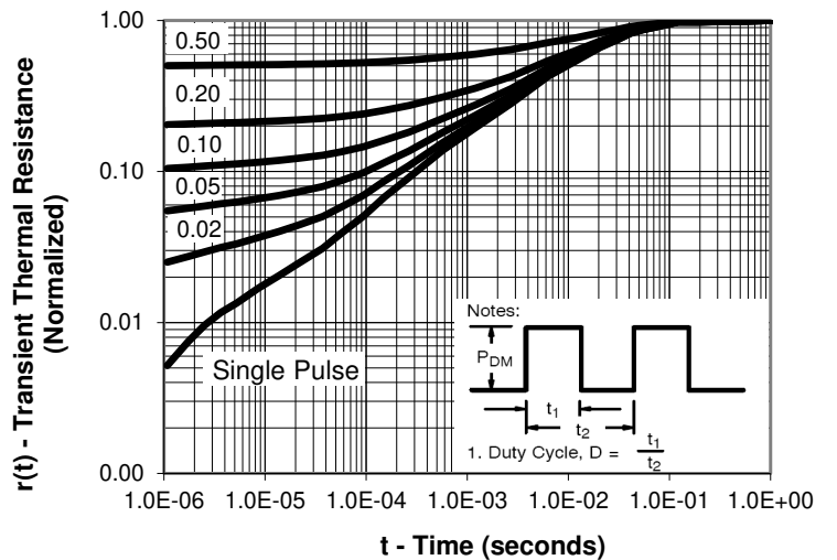
TO-247 Transient Thermal Response, Junction-to-Ambient
