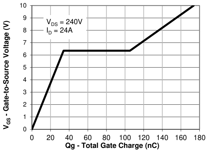
Gate Charge
