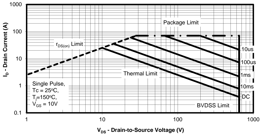
Maximum Rated Forward Biased Safe Operating Area
