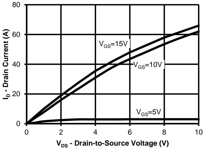
Output Characteristics
