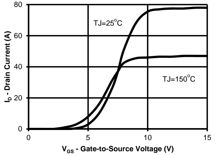
Transfer Characteristics
