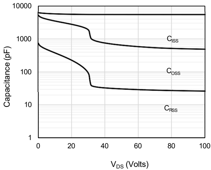
Figure 9: Capacitance Characteristics
