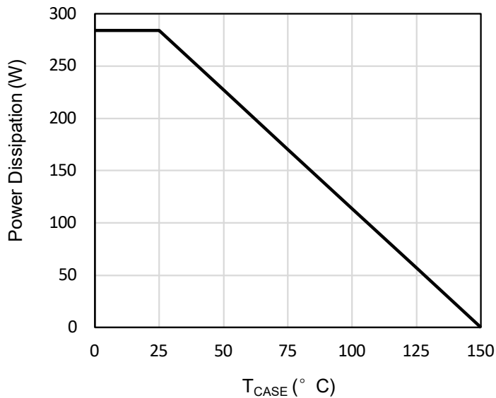
Figure 11: Power De-rating
