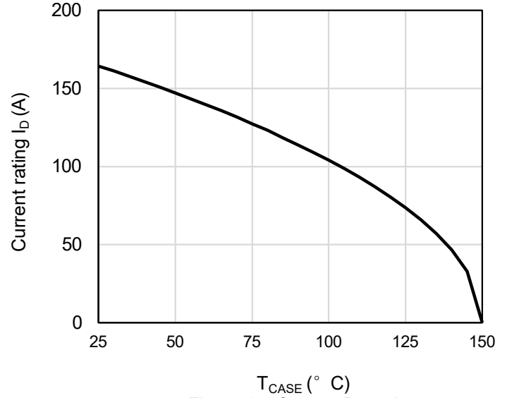
Figure 12: Current De-rating
