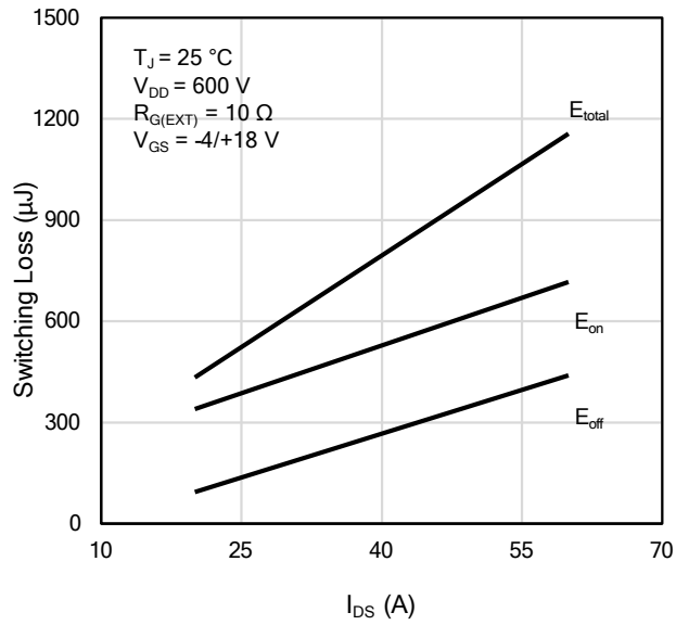
Figure 25: Clamped Inductive Switching Energy vs. Drain Current ( V_{DD} = 600\text{ V} )
