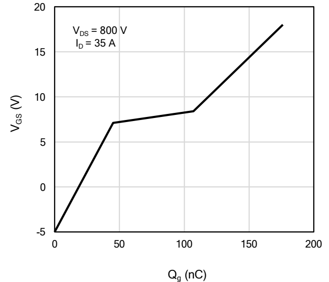
Figure 12: Gate-Charge Characteristics
