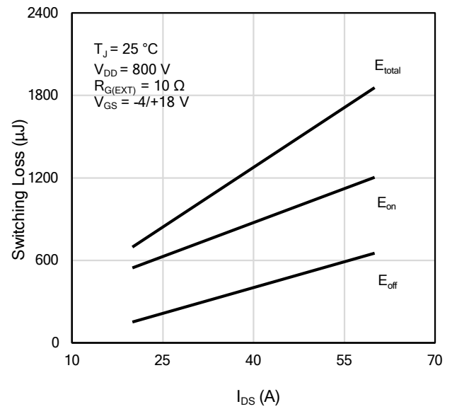
Figure 26: Clamped Inductive Switching Energy vs. Drain Current ( V_{DD} = 800\text{ V} )
