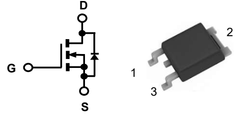
DPAK (TO252) 1=Gate, 2=Drain, 3=Source.
