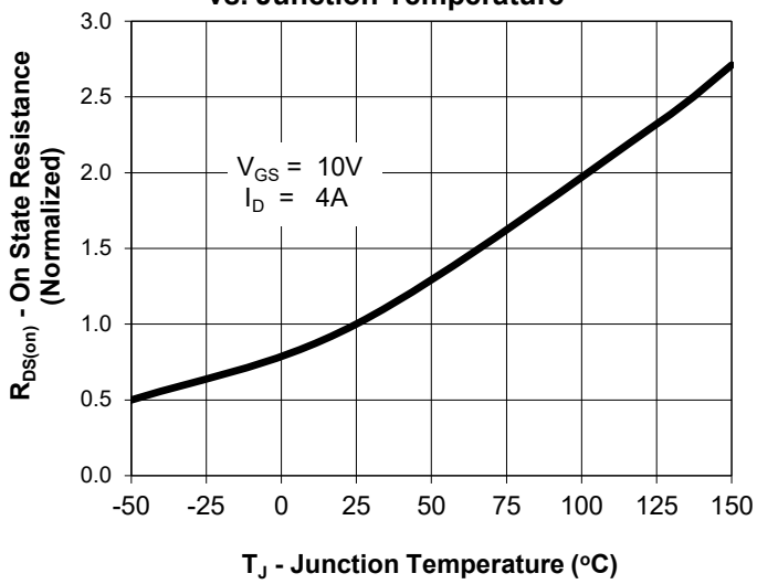
Drain-Source On State Resistance vs. Junction Temperature
