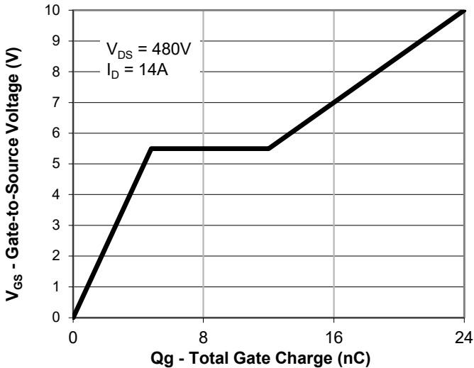
Gate Charge
