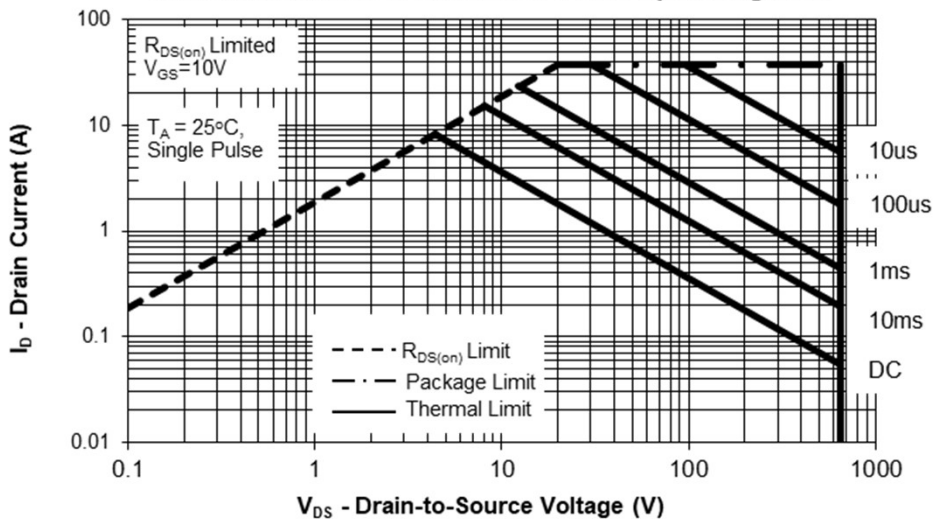
Full Pak TO-220 Package Maximum Rated Forward Biased Safe Operating Area
