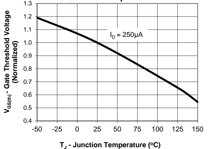
Gate Threshold Voltage vs. Junction Temperature
