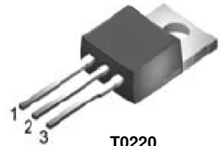
TO220 Standard Metal Heatsink 1=Gate, 2=Drain, 3=Source.
