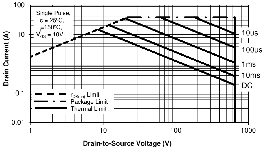
Maximum Rated Forward Biased Safe Operating Area
